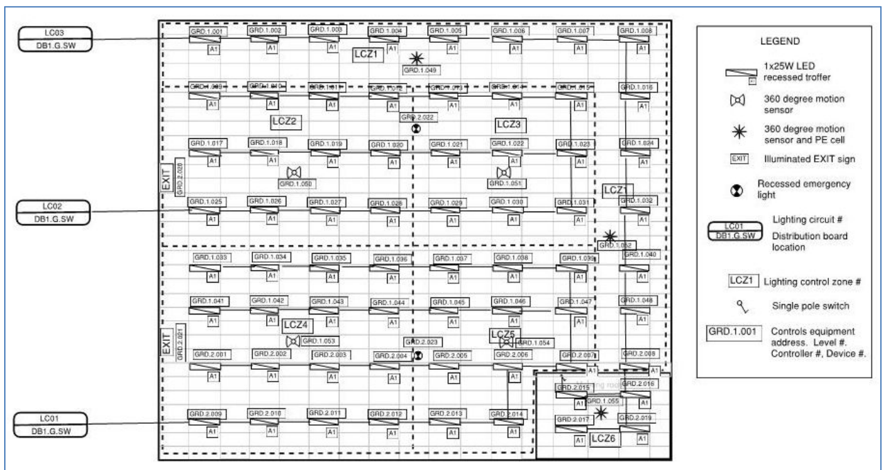
Figure 27: Detailed plan of a soft wired controls system
