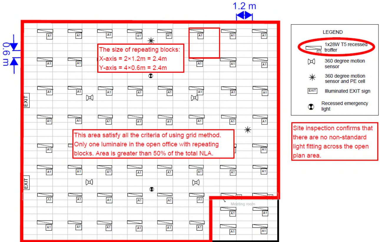
Figure 11: Sample marked up RCP for Grid Method
