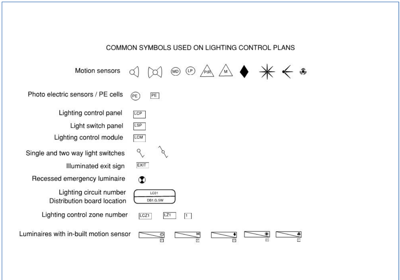
Figure 30: Common symbols used on lighting control plans
