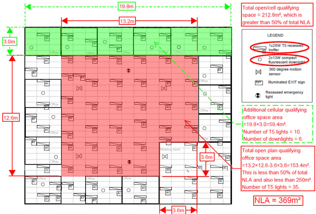
Figure 17: Sample marked up RCP for Aggregate Method 2
