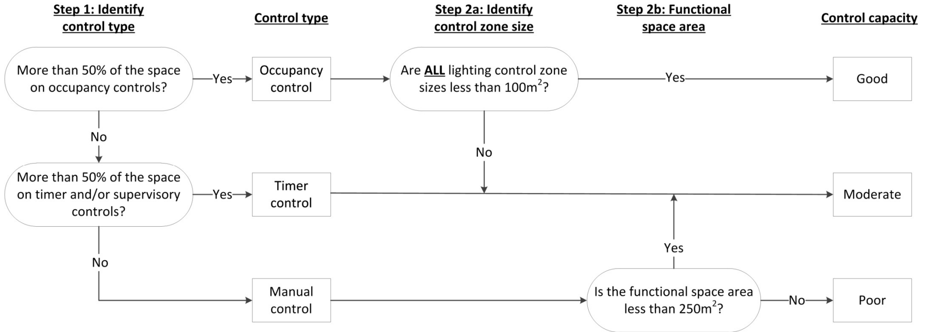
Figure 7: Lighting control assessment methodology flow chart
