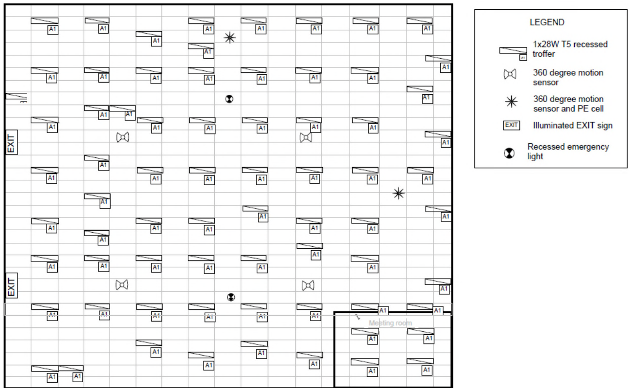
Figure 13: Sample RCP for Aggregate Method 1
