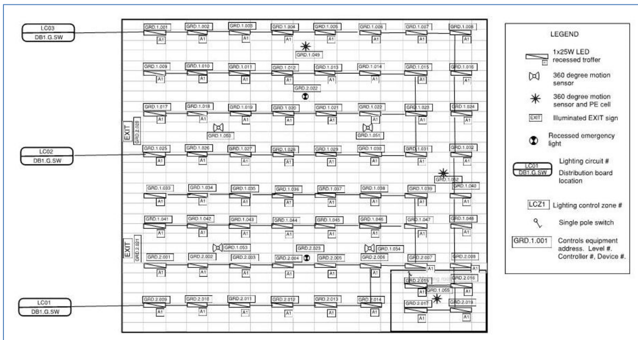
Figure 28: Plan of a soft wired controls system showing lighting circuits, but no zones
